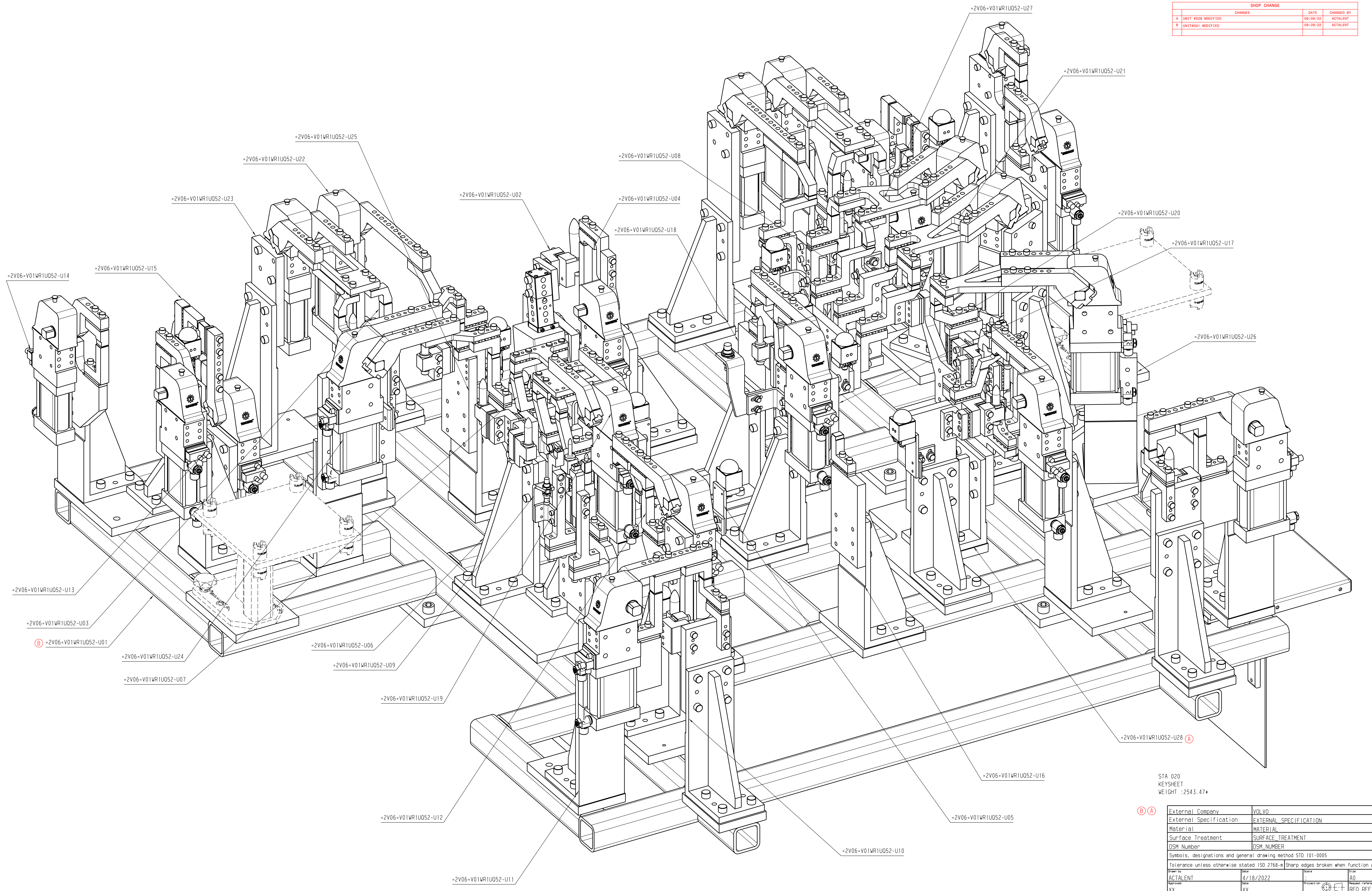
ISO VIEW -1
