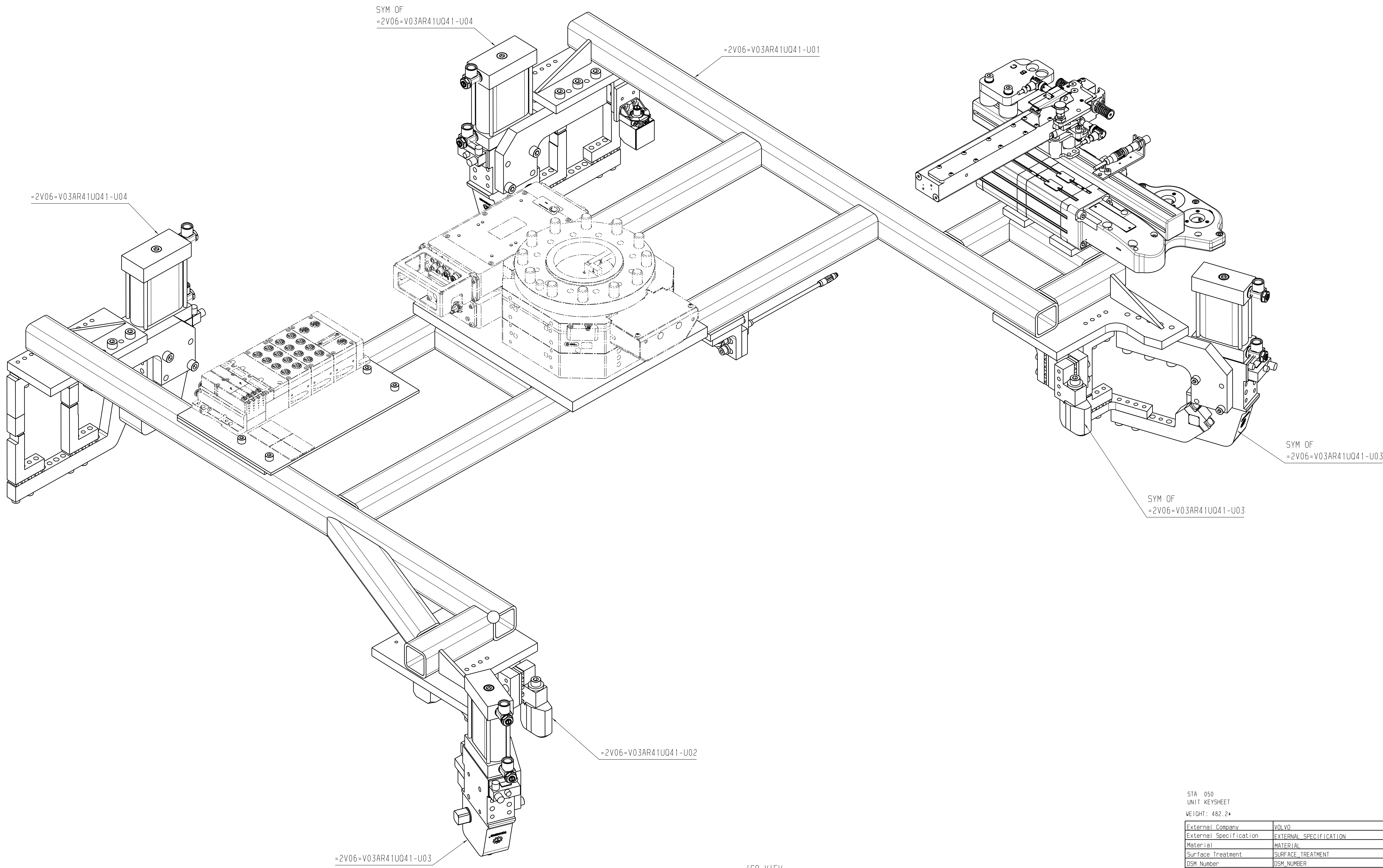
ISO VIEW
