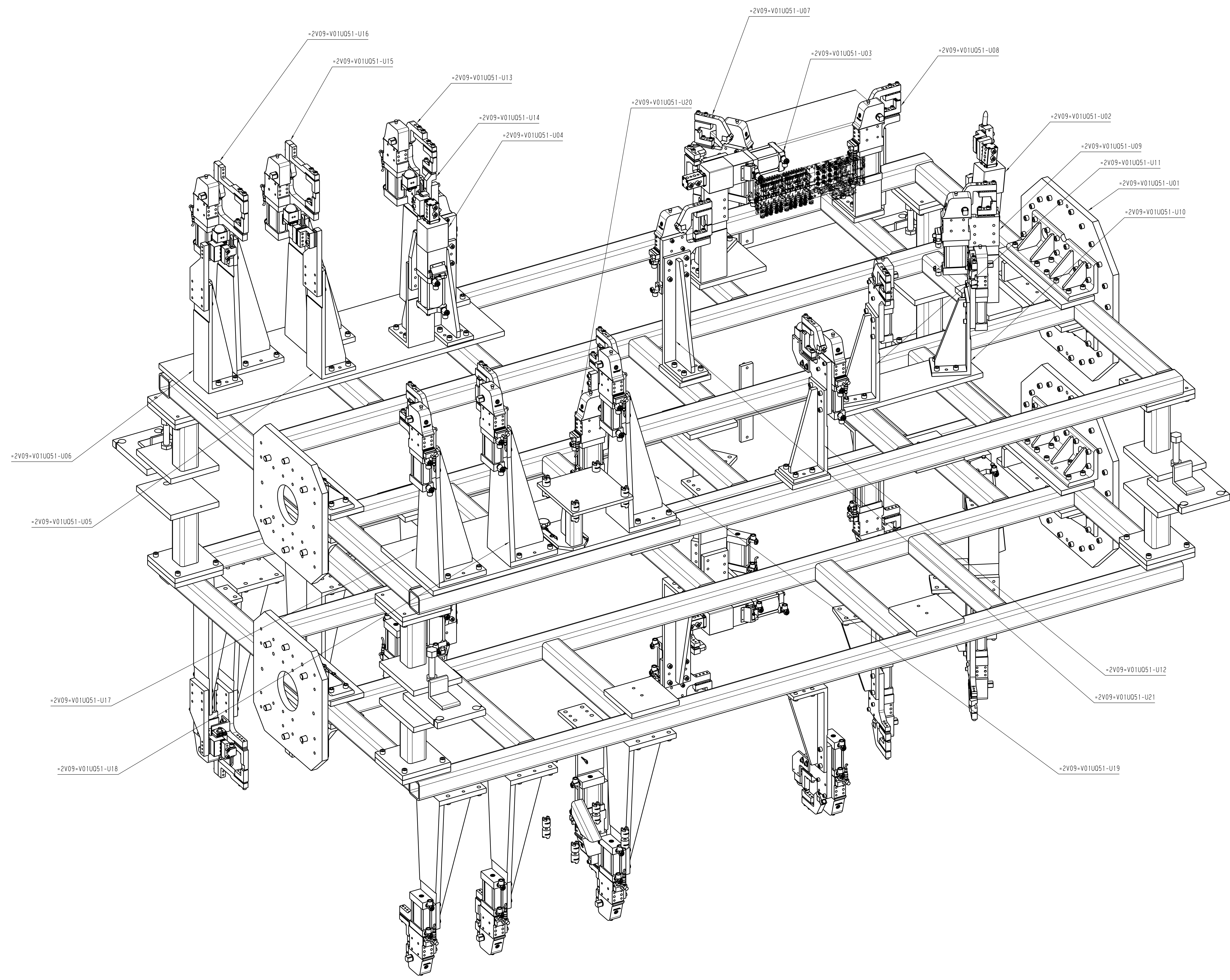
ISO VIEW-1
