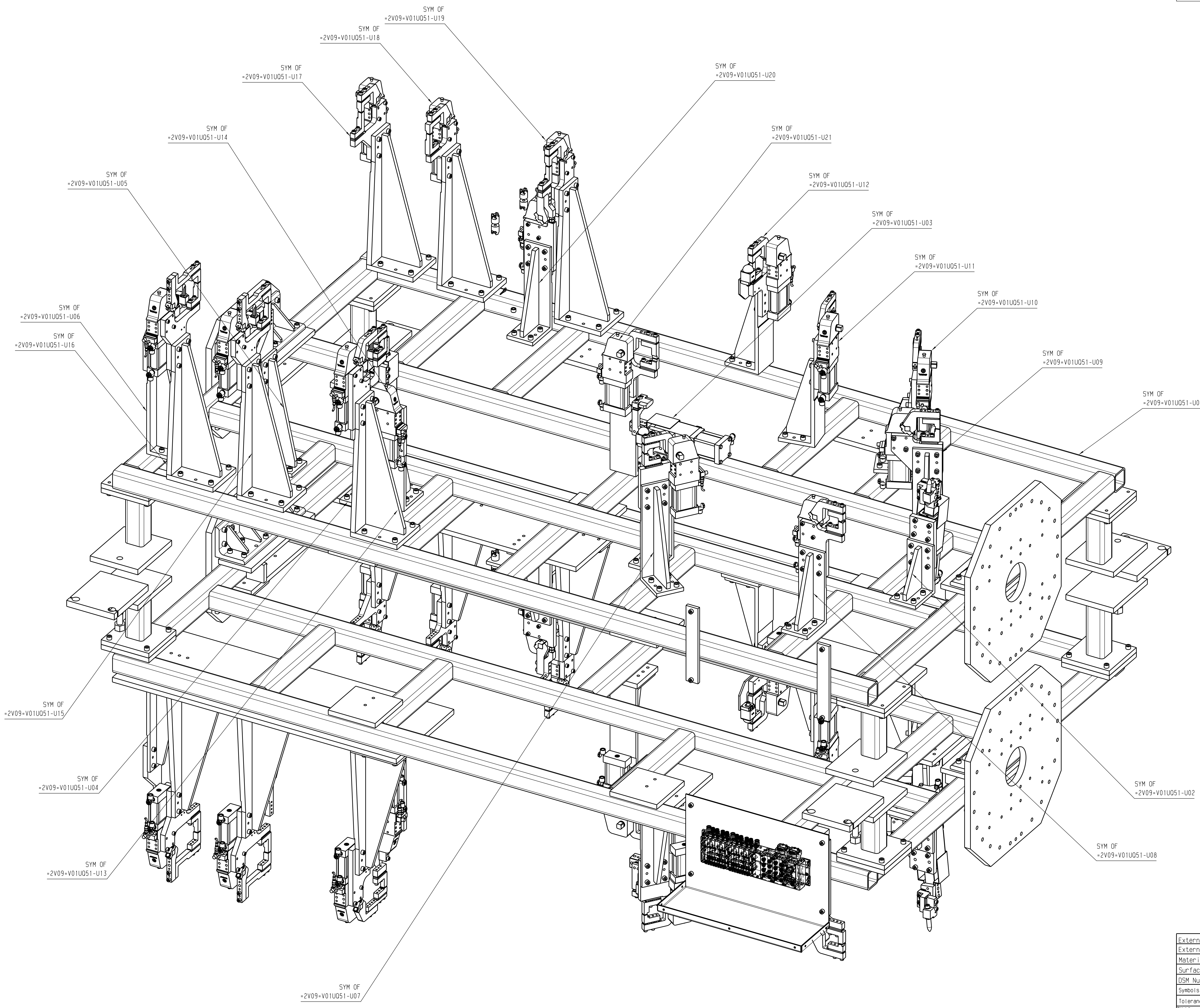
ISO VIEW-2
