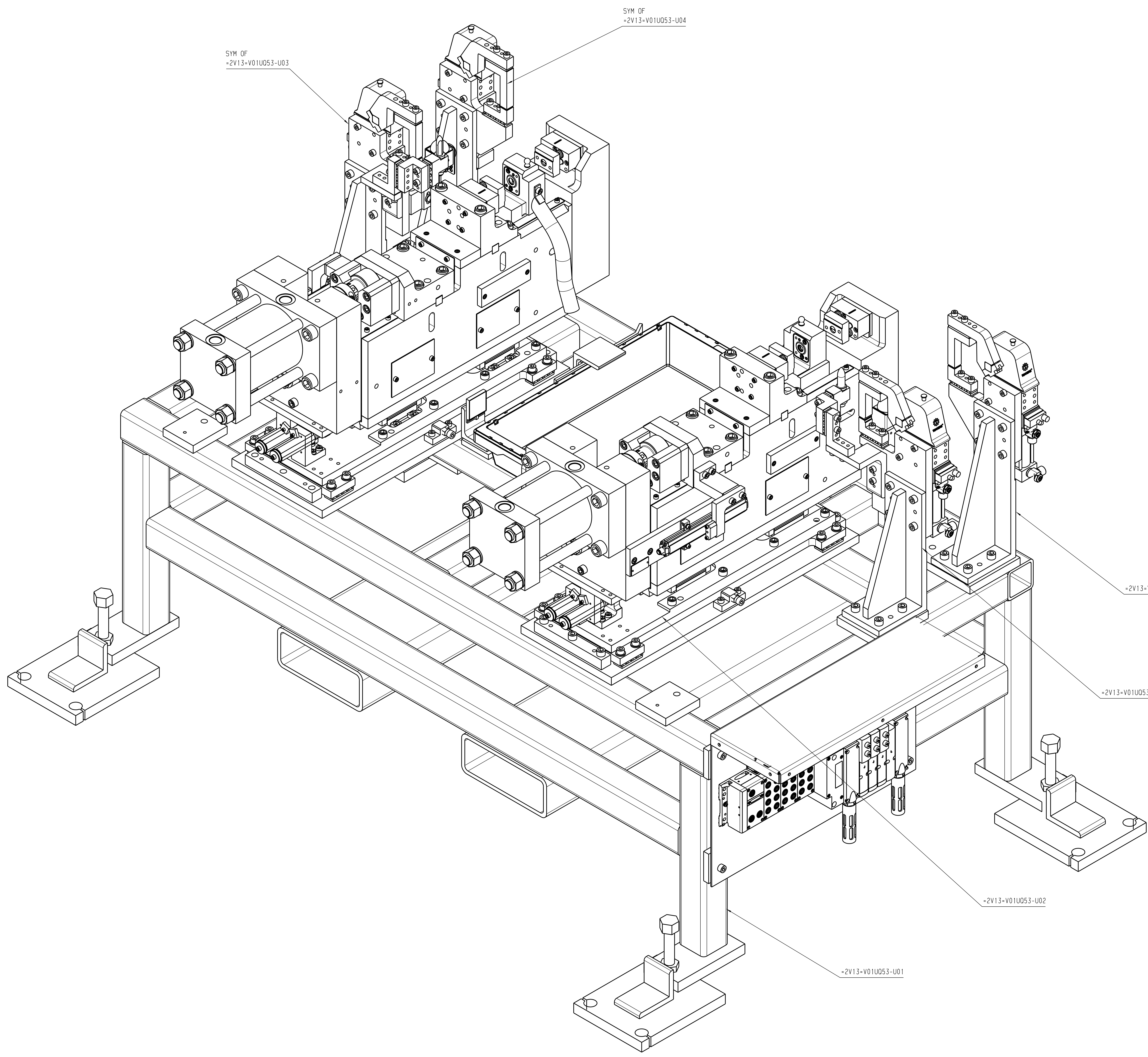
ISO VIEW-1
