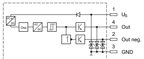
Outputs: Open collector
