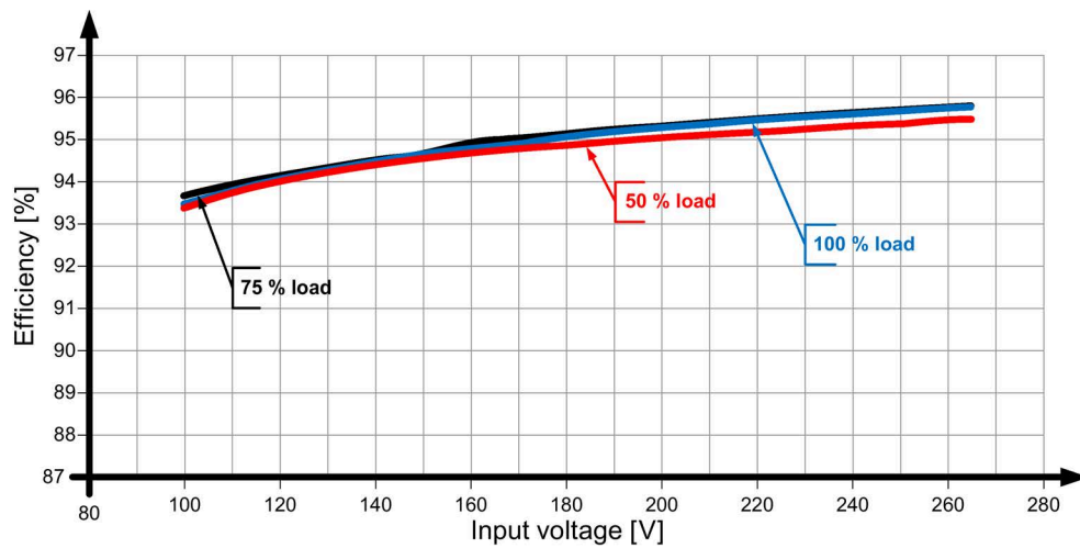
Figure 6-21 Efficiency 6EP3336-7SB00-3AX0 and 6EP3336-7SC00-3AX0
