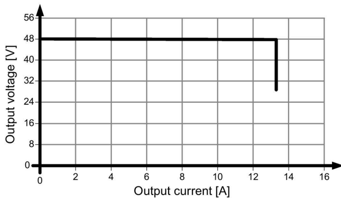
Figure 6-10 Output characteristic 6EP3346-7SB00-3AX0 single operation
