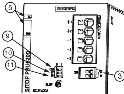
Figure 2-6 Signaling, signaling contact
