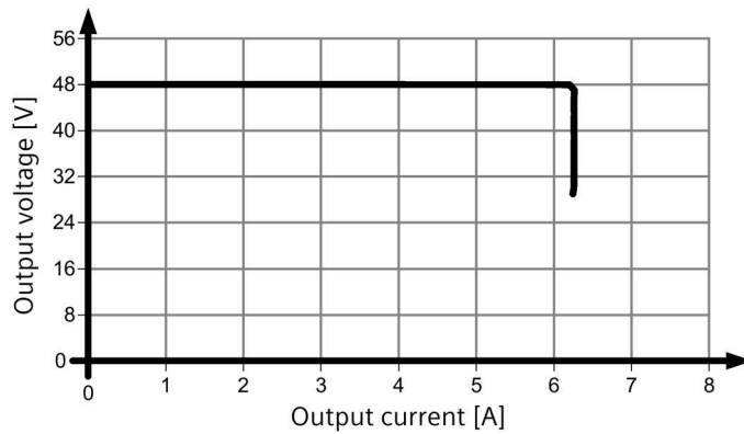
Figure 6-9 Output characteristic 6EP3344-7SB00-3AX0 single operation
