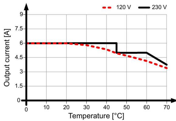
Figure 4-29 Mounting position 5
