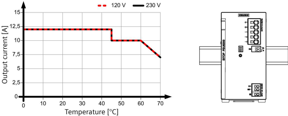
Figure 4-8 6EP3346-7SB00-3AX0 output current for the standard mounting position
