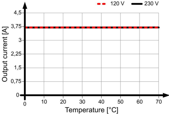
Figure 4-22 Mounting position 3
