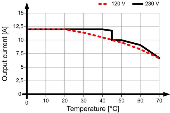
Figure 4-30 Mounting position 1
