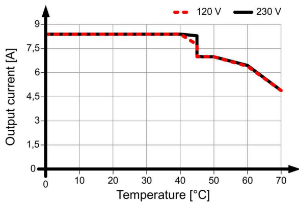
Figure 4-12 Mounting position 3
