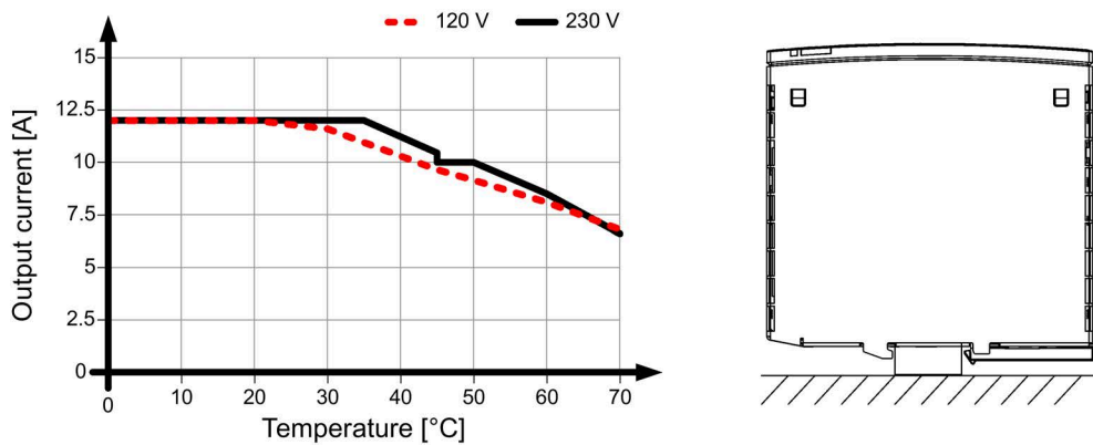
Figure 4-33 Mounting position 4
