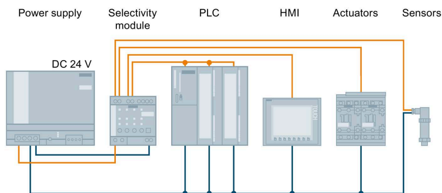
Figure 9-4 Electronic protection of 24 V loads using the SITOP PSE200U selectivity module
