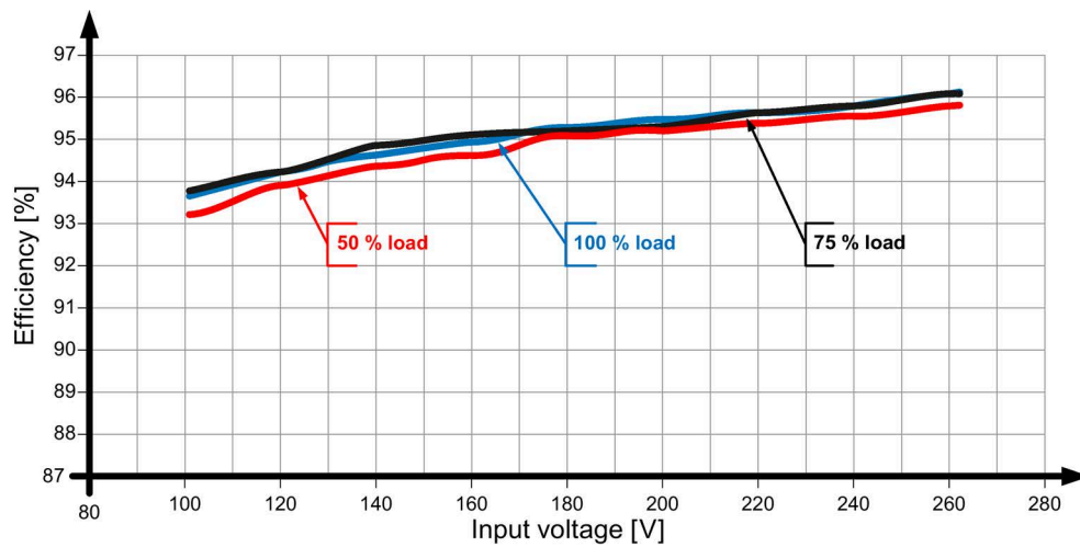
Figure 6-23 Efficiency 6EP3346-7SB00-3AX0
