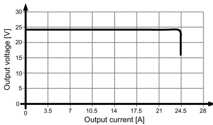
Figure 6-8 Output characteristic 6EP3336-7SB00-3AX0 and 6EP3336-7SC00-3AX0 single operation
