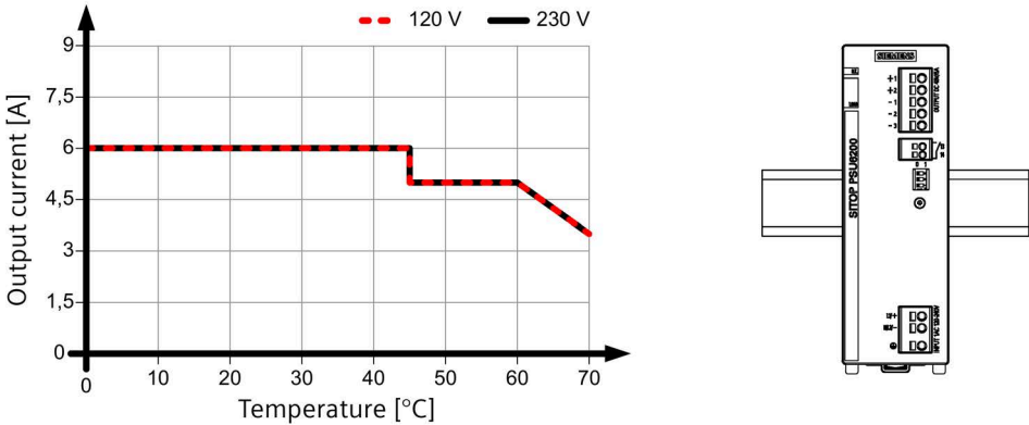
Figure 4-7 6EP3344-7SB00-3AX0 output current for the standard mounting position
