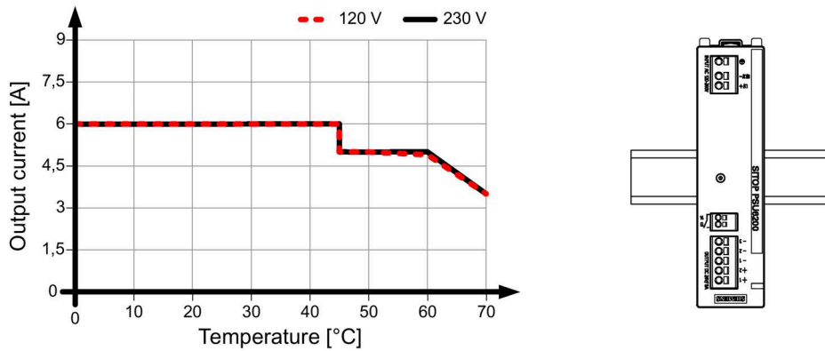
Figure 4-27 Mounting position 3
