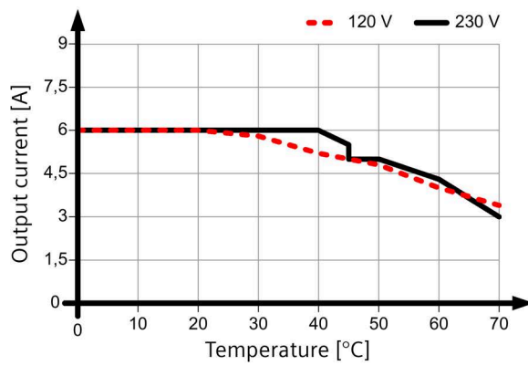
Figure 4-43 Mounting position 4
