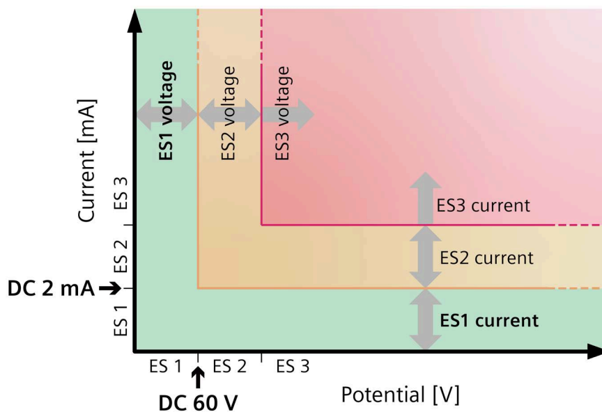
Figure 9-2 Representation of the ES limit values for voltage and current
