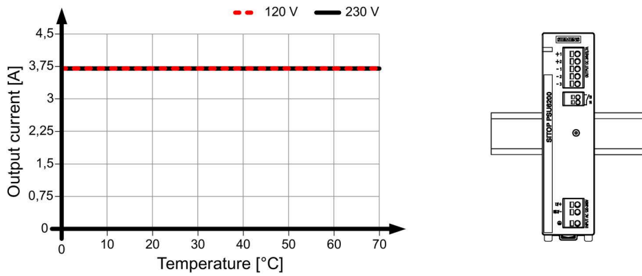
Figure 4-3 6EP3333-7LB00-0AX0 output current for the standard mounting position
