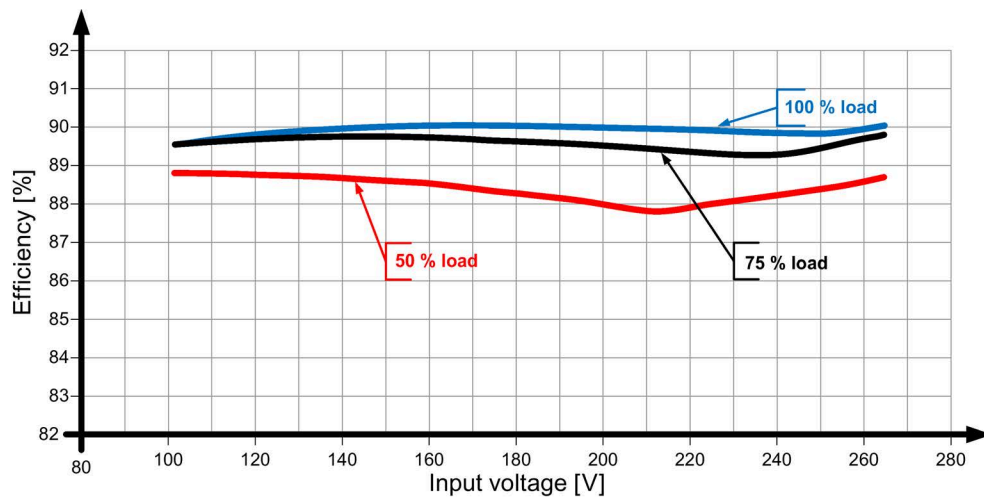
Figure 6-17 Efficiency 6EP3324-7SB00-3AXO
