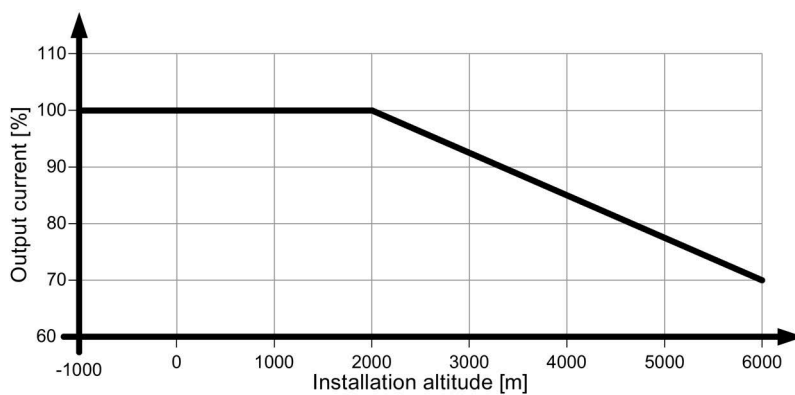
Figure 4-9 Mounting height derating
