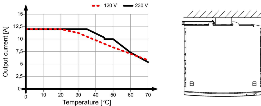
Figure 4-34 Mounting position 5
