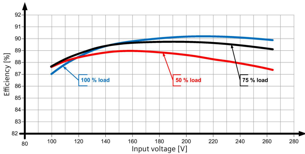
Figure 6-19 Efficiency 6EP3333-7SB00-0AX0 and 6EP3333-7SC00-0AX0
