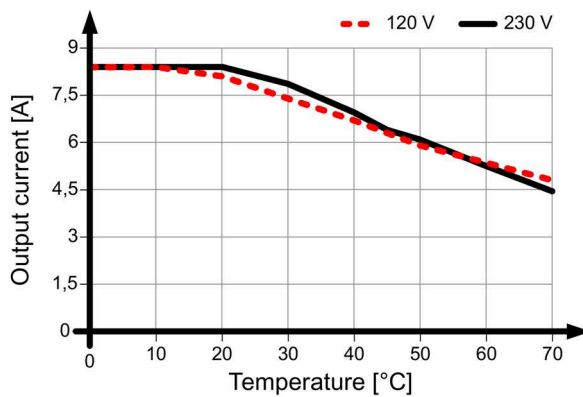
Figure 4-10 Mounting position 1
