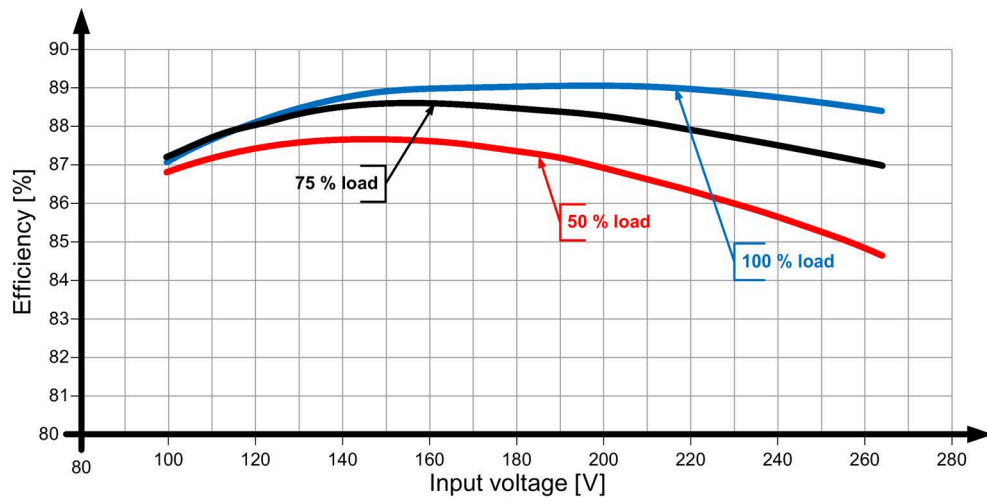
Figure 6-18 Efficiency 6EP3333-7LB00-0AX0
