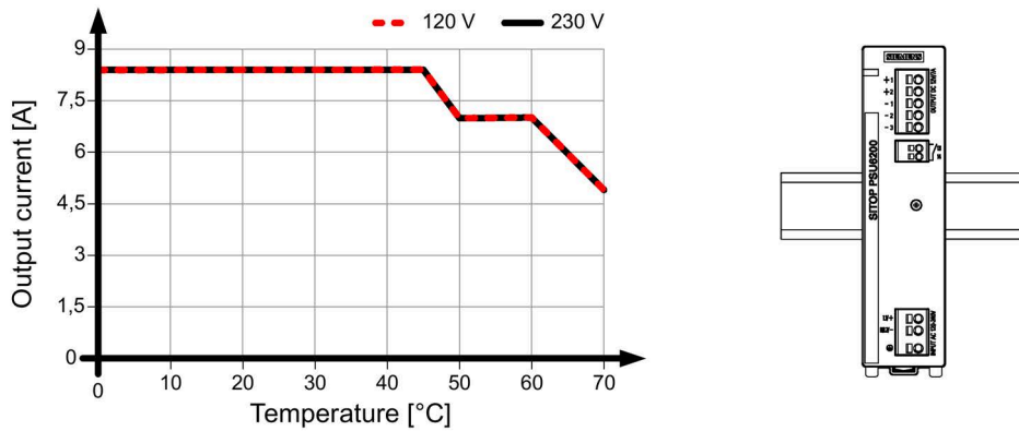
Figure 4-1 6EP3323-7SB00-0AX0 output current for the standard mounting position
