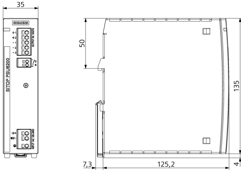
Figure 2-9 Dimension drawing 6EP3323-7SB00-0AX0, 6EP3333-7LB00-0AX0, 6EP3333-7SB00-0AX0 and 6EP3333-7SC00-0AX0
