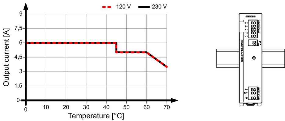
Figure 4-4 6EP3333-7SB00-0AX0 and 6EP3333-7SC00-0AX0 output current for the standard mounting position
