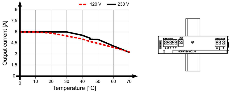
Figure 4-25 Mounting position 1
