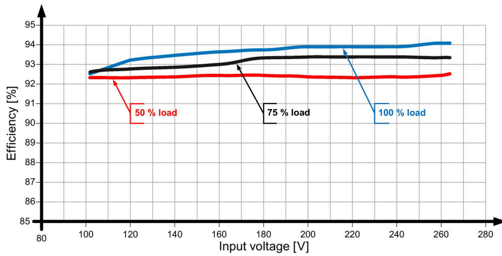
Figure 6-22 Efficiency 6EP3344-7SB00-3AX0
