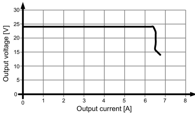
Figure 6-6 Output characteristic 6EP3333-7SB00-0AX0 and 6EP3333-7SC00-0AX0 single operation
