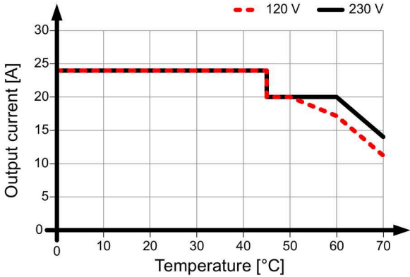
Figure 4-36 Mounting position 2
