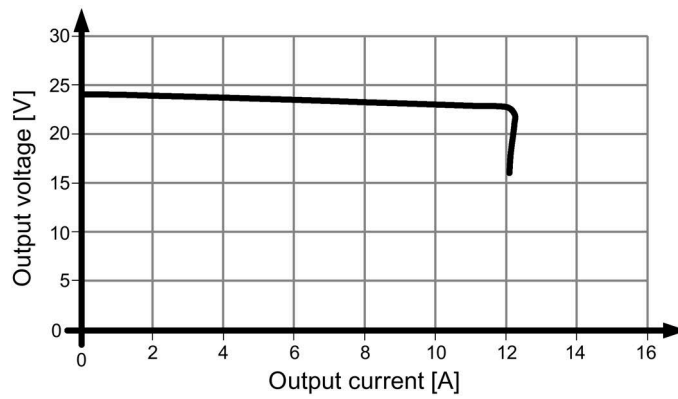
Figure 6-12 Output characteristic 6EP3334-7SB00-3AX0 and 6EP3334-7SC00-3AX0 parallel operation
