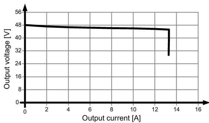
Figure 6-15 Output characteristic 6EP3346-7SB00-3AX0 parallel operation
