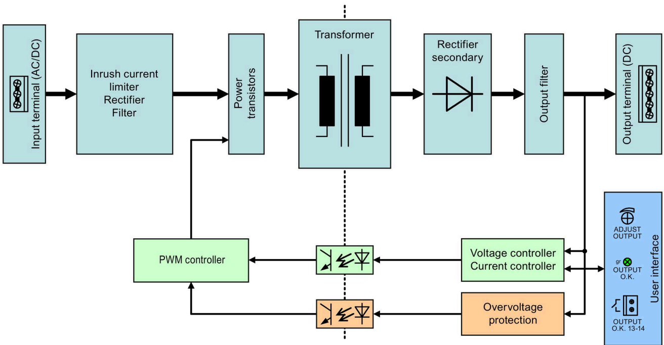
Figure 2-7 Block diagram 12 V/7 A and 24 V/3.7 A, 24 V/5 A devices
