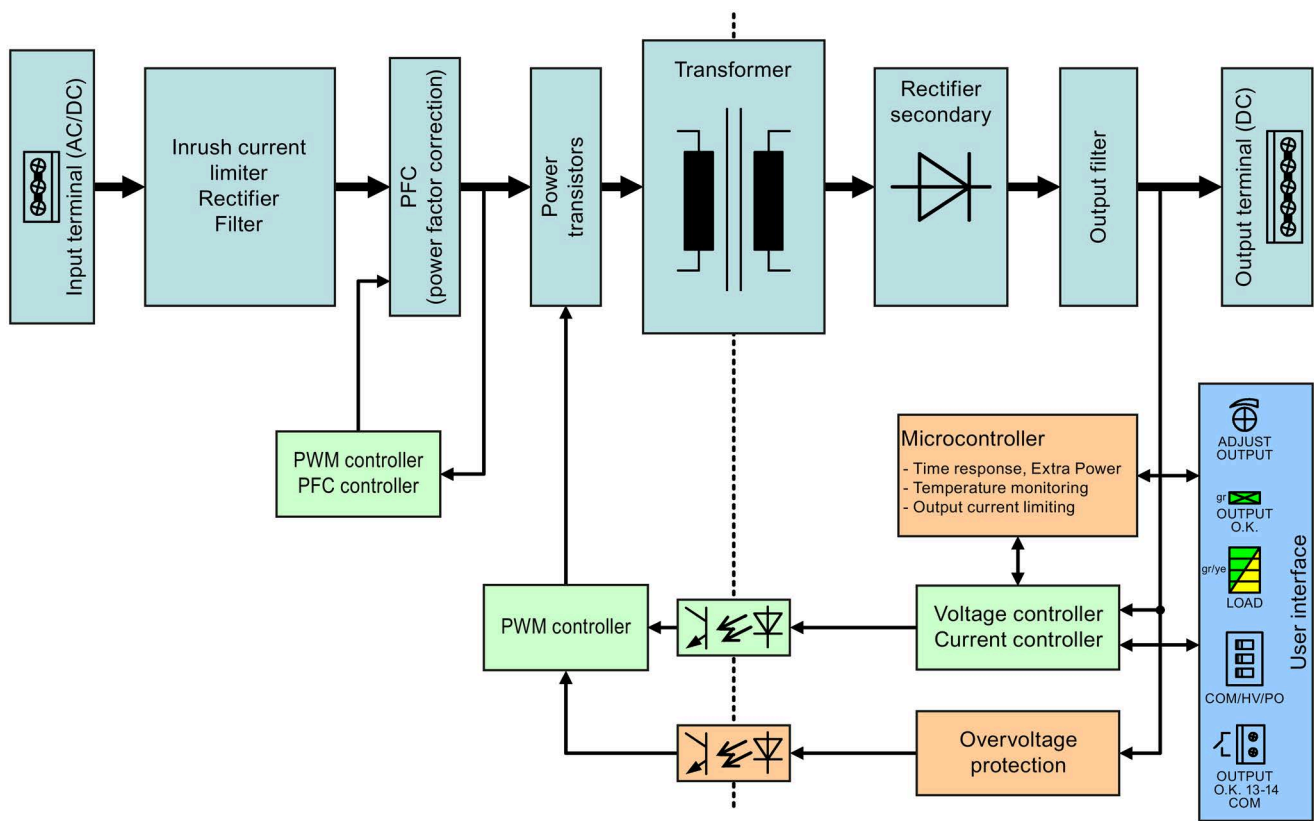
Figure 2-8 Block diagram 12 V/12 A and 24 V/10 A, 24 V/20 A and 48 V/5 A, 48 V/10 A devices
