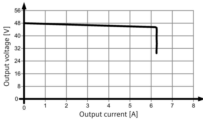
Figure 6-14 Output characteristic 6EP3344-7SB00-3AX0 parallel operation
