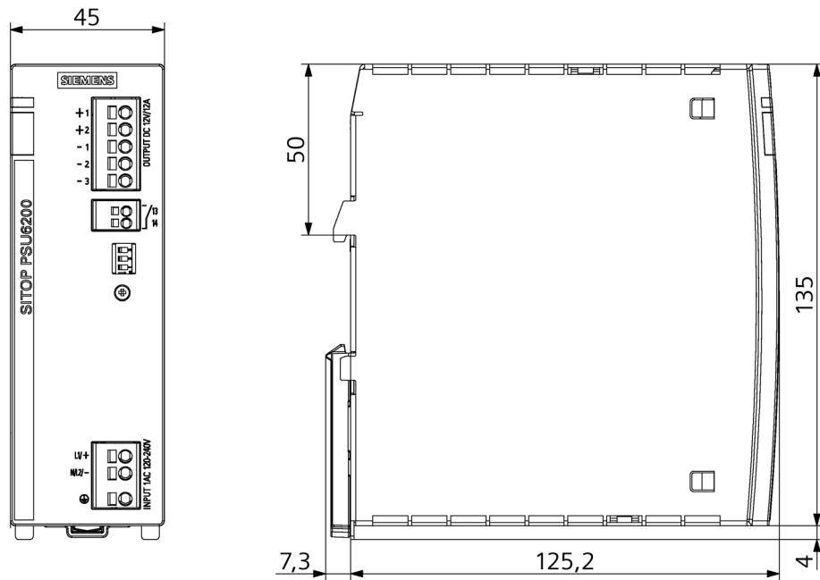
Figure 2-10 Dimension drawing 6EP3324-7SB00-3AX0, 6EP3334-7SB00-3AX0, 6EP3344-7SB00-3AX0 and 6EP3334-7SC00-3AX0
