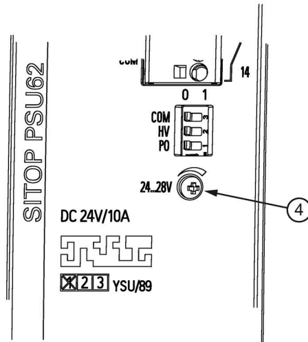
Figure 2-4 Potentiometer
