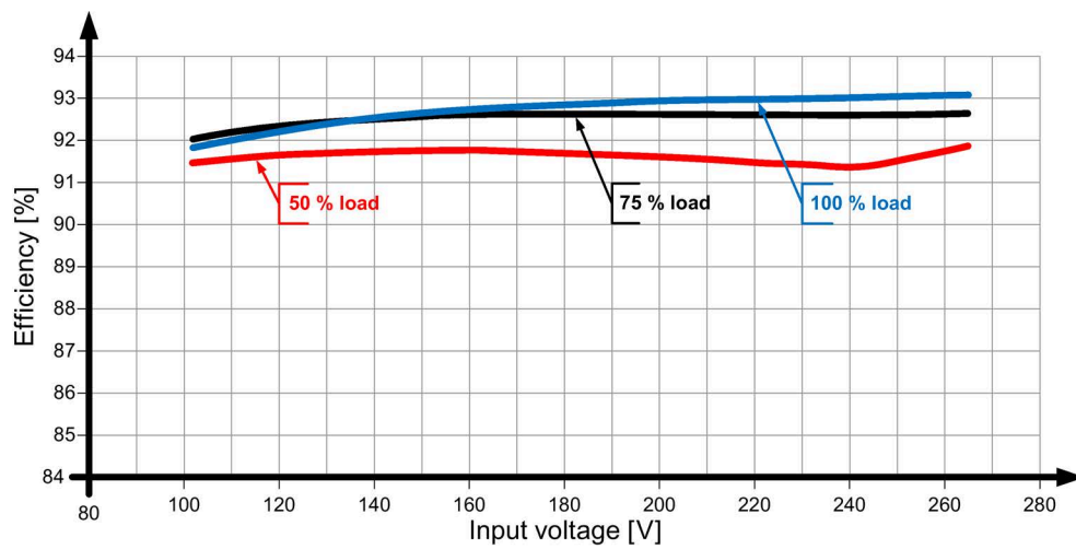
Figure 6-20 Efficiency 6EP3334-7SB00-3AX0 and 6EP3334-7SC00-3AX0
