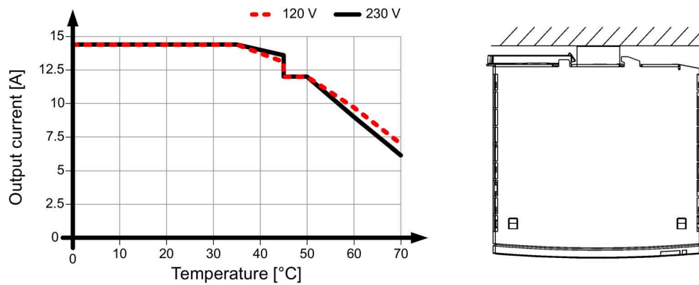
Figure 4-19 Mounting position 5
