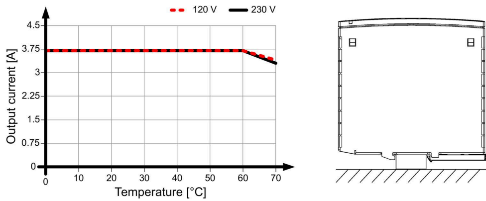
Figure 4-23 Mounting position 4
