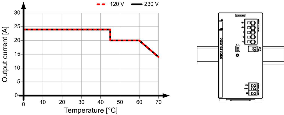
Figure 4-6 6EP3336-7SB00-3AX0 and 6EP3336-7SC00-3AX0 output current for the standard mounting position
