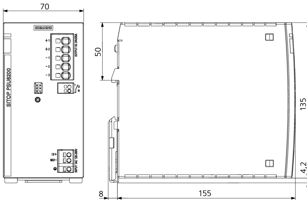
Figure 2-11 Dimension drawing 6EP3336-7SB00-3AX0, 6EP3346-7SB00-3AX0 and 6EP3336-7SC00-3AX0
