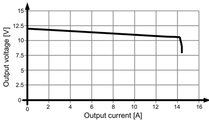
Figure 6-11 Output characteristic 6EP3324-7SB00-3AX0 parallel operation
