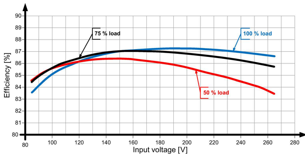
Figure 6-16 Efficiency 6EP3323-7SB00-0AXO
