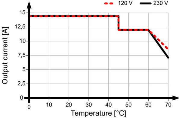
Figure 4-17 Mounting position 3
