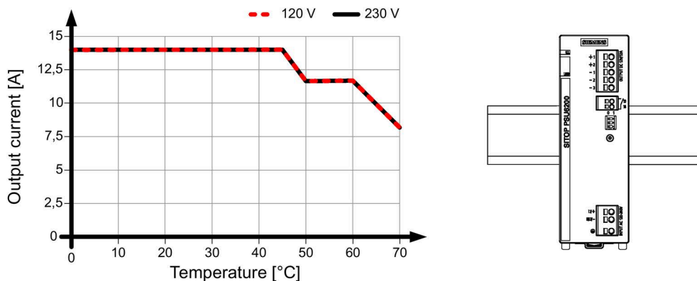
Figure 4-2 6EP3324-7SB00-3AX0 output current for the standard mounting position
