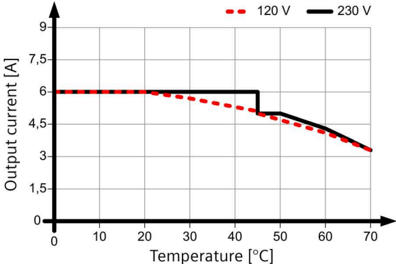
Figure 4-41 Mounting position 2
