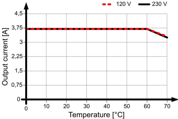
Figure 4-20 Mounting position 1
