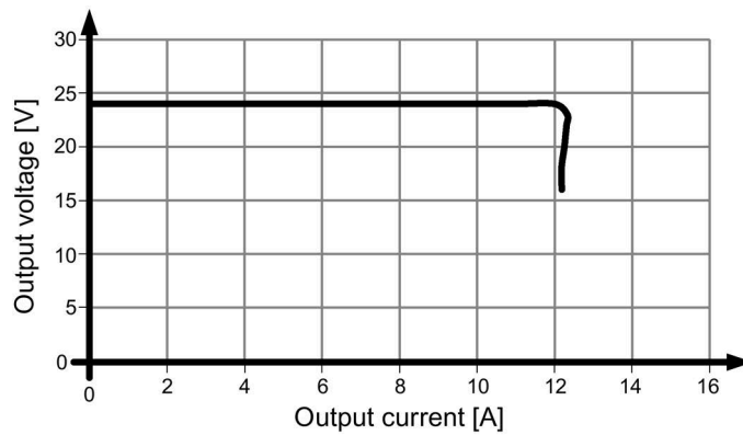
Figure 6-7 Output characteristic 6EP3334-7SB00-3AX0 and 6EP3334-7SC00-3AX0 single operation
