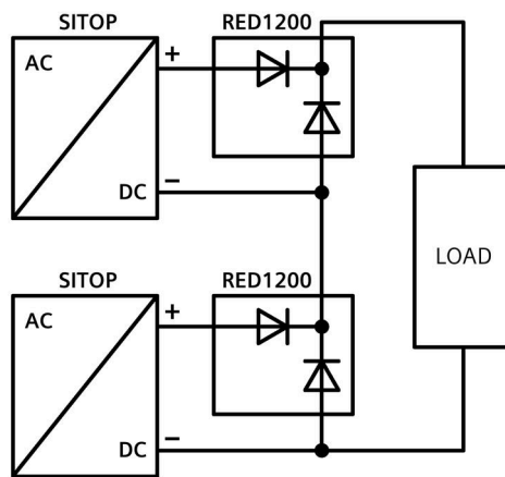
Figure 9-3 Series connection
