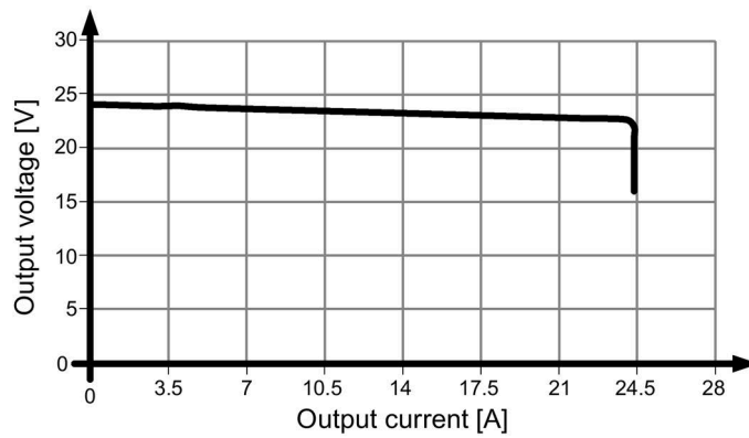
Figure 6-13 Output characteristic 6EP3336-7SB00-3AX0 and 6EP3336-7SC00-3AX0 parallel operation
