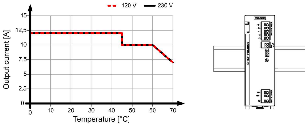
Figure 4-5 6EP3334-7SB00-3AX0 and 6EP3334-7SC00-3AX0 output current for the standard mounting position
