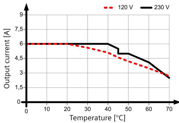
Figure 4-44 Mounting position 5
