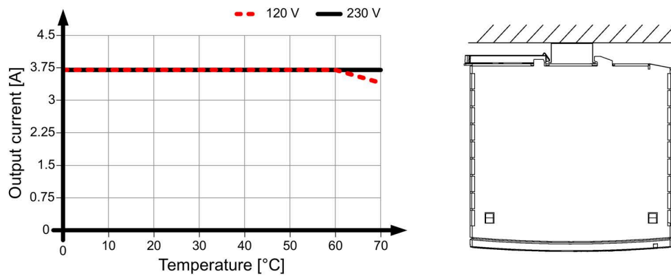
Figure 4-24 Mounting position 5
