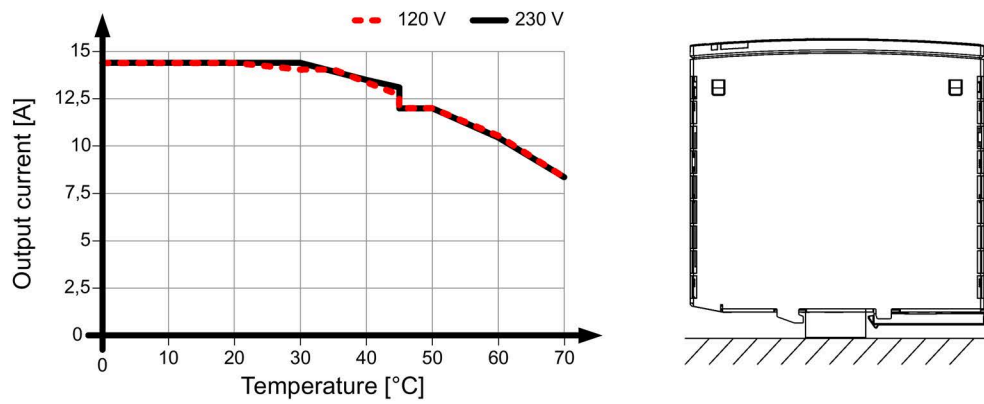
Figure 4-18 Mounting position 4
