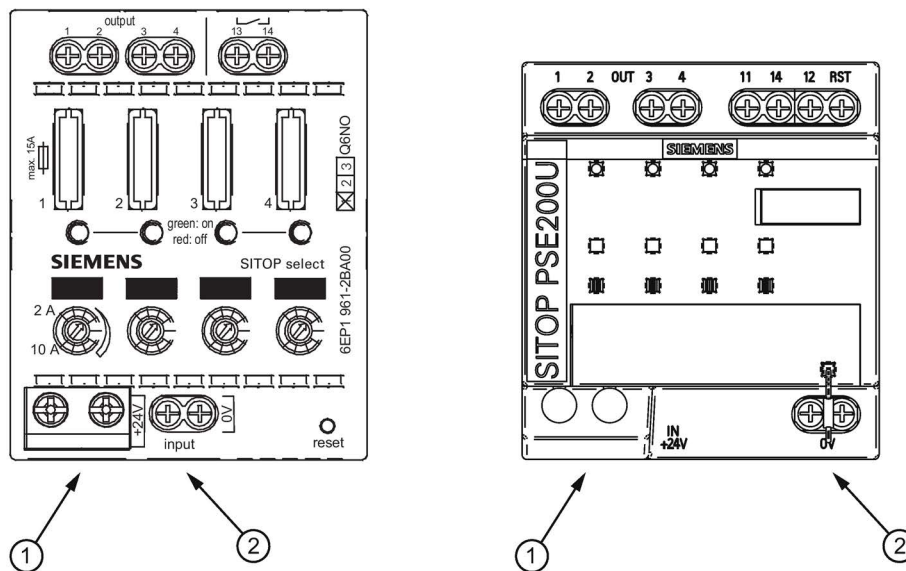
Figure 5-1 Input connection
