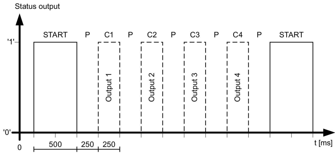
Figure 2-5 Status signaling
