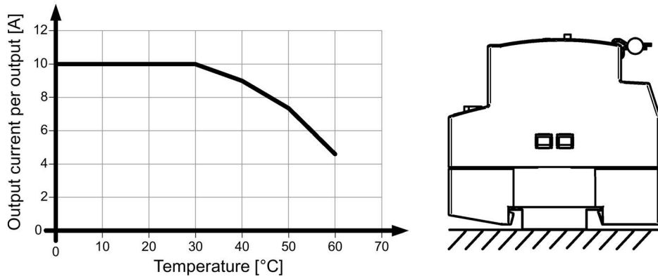
Figure 4-18 Mounting position (4)
