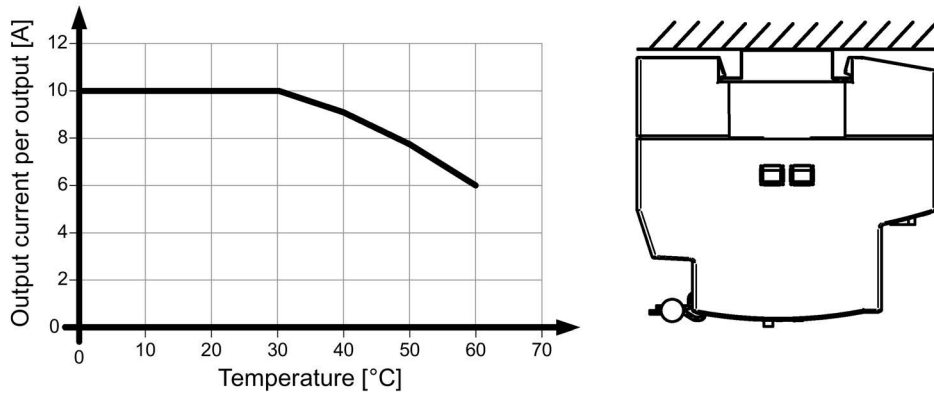
Figure 4-19 Mounting position (5)
