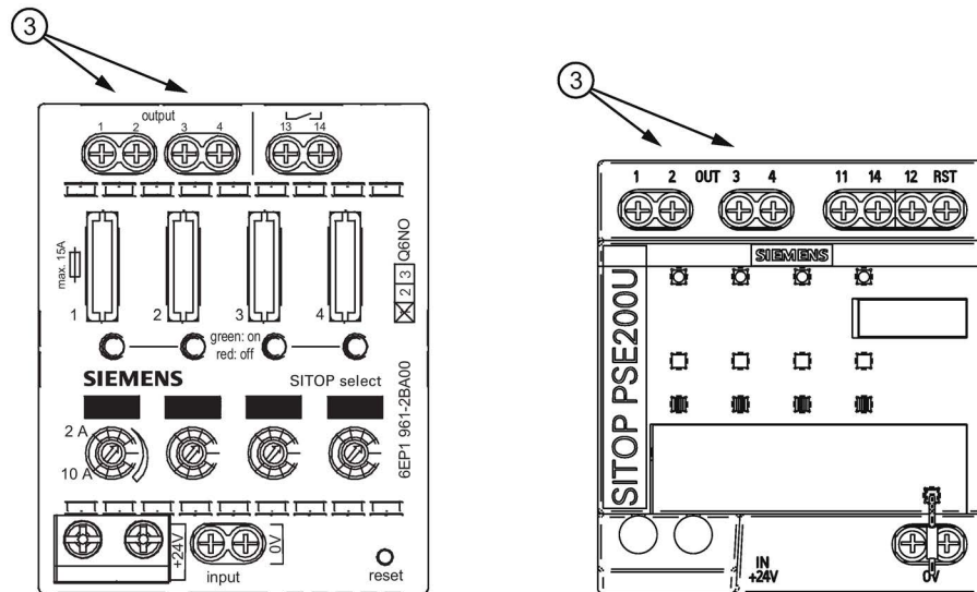
Figure 5-2 Output connection
