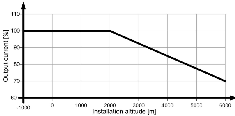
Figure 4-4 Mounting height derating
