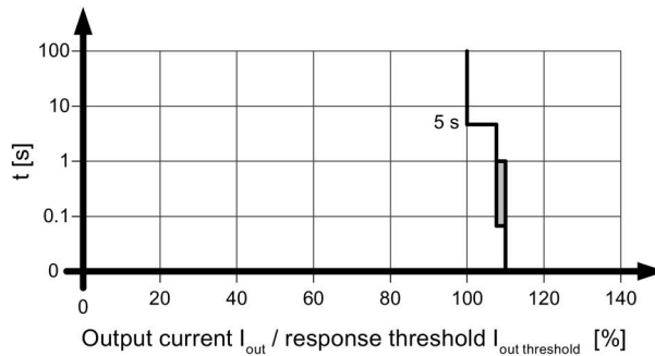
Figure 2-12 Shutdown characteristic 6EP1961-2BA51, -2BA61
