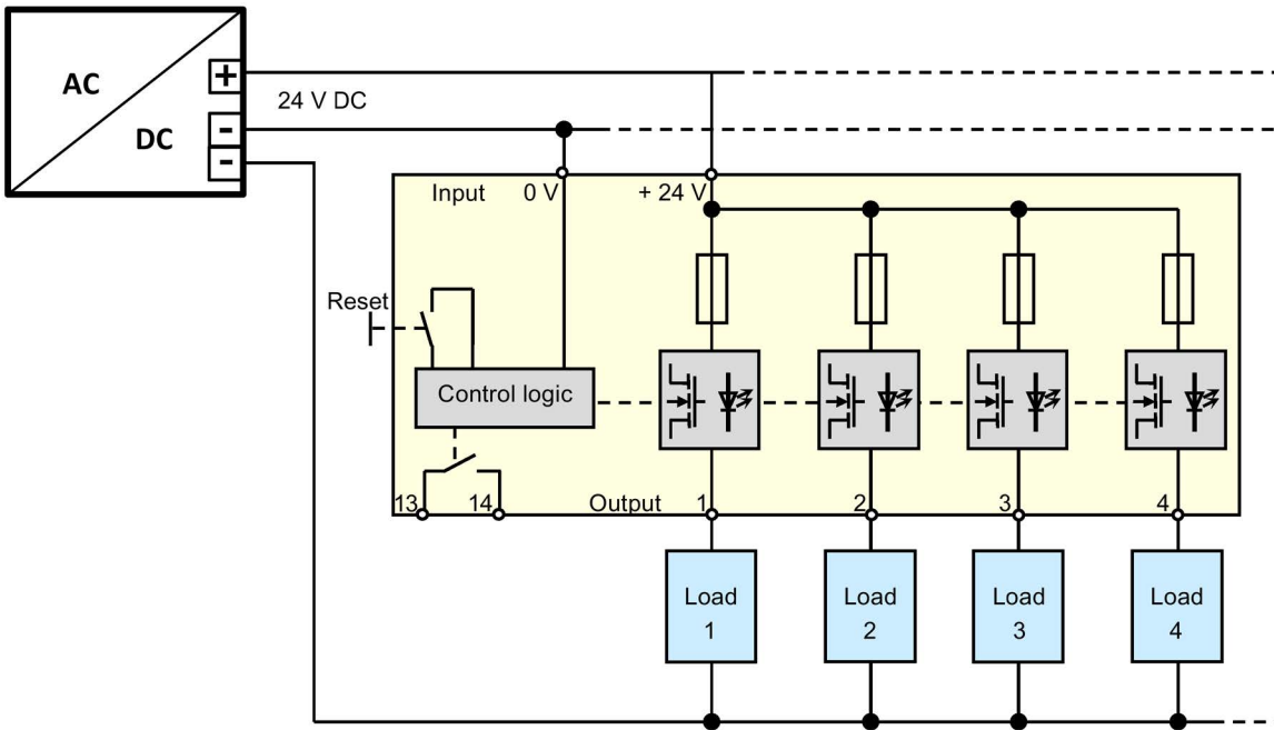
Figure 2-16 Block diagram of the 6EP1961-2BA00
