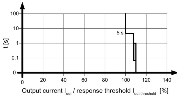
Figure 6-4 Shutdown characteristic 6EP1961-2BA51, -2BA61
