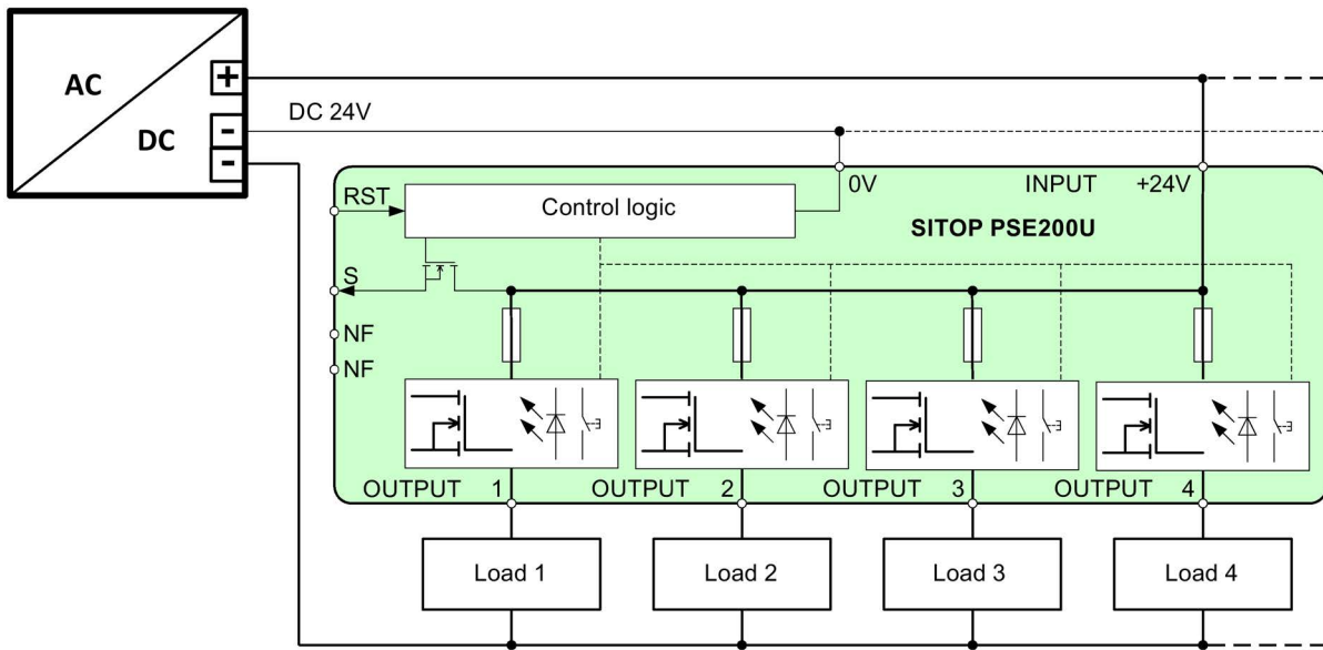
Figure 2-18 Block diagram 6EP1961-2BA31, 6EP1961-2BA41 and 6EP1961-2BA61
