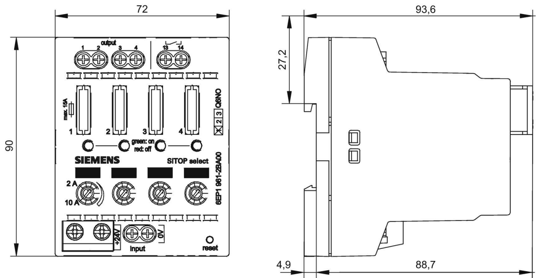
Figure 2-19 Dimension drawing 6EP1961-2BA00
