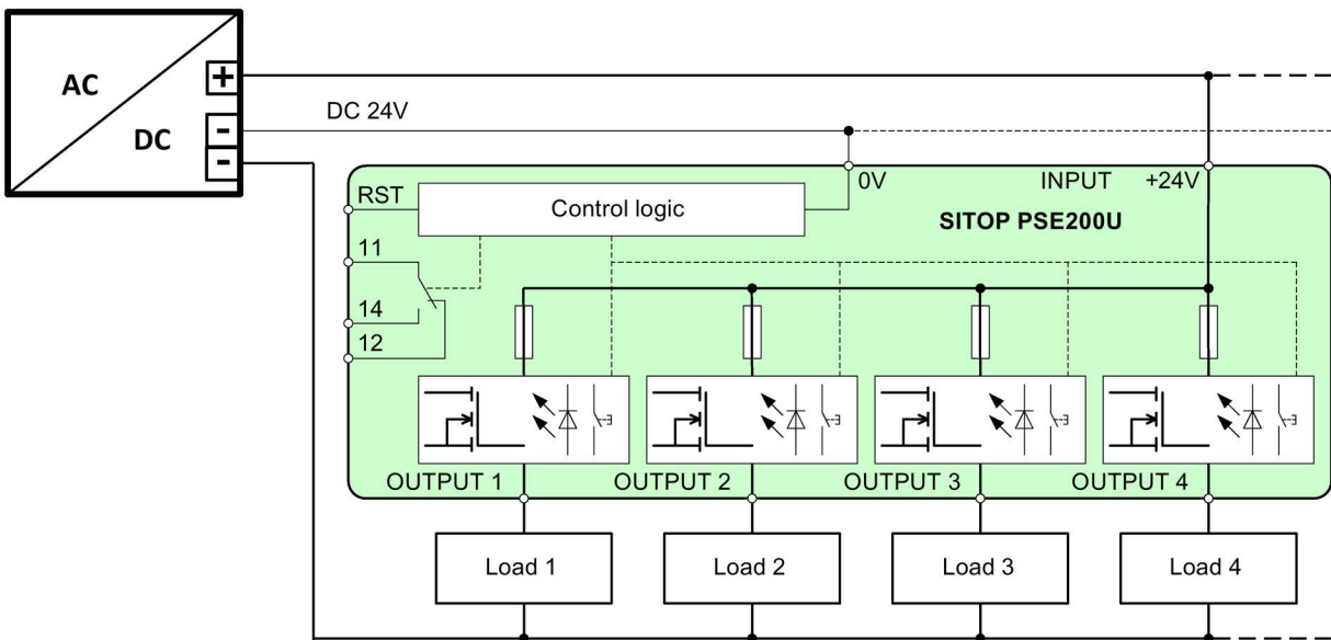
Figure 2-17 Block diagram for 6EP1961-2BA11, 6EP1961-2BA21 and 6EP1961-2BA51
